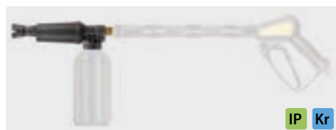
M22 M. Foam injector lance with regulator and bottle. Max. 300 bar / 80 °C
